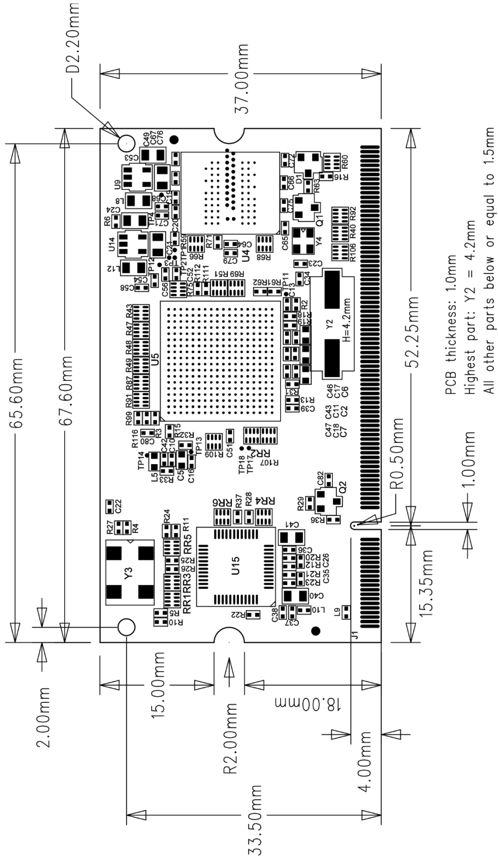
Figure 2: PM9G45 v1.3 top
