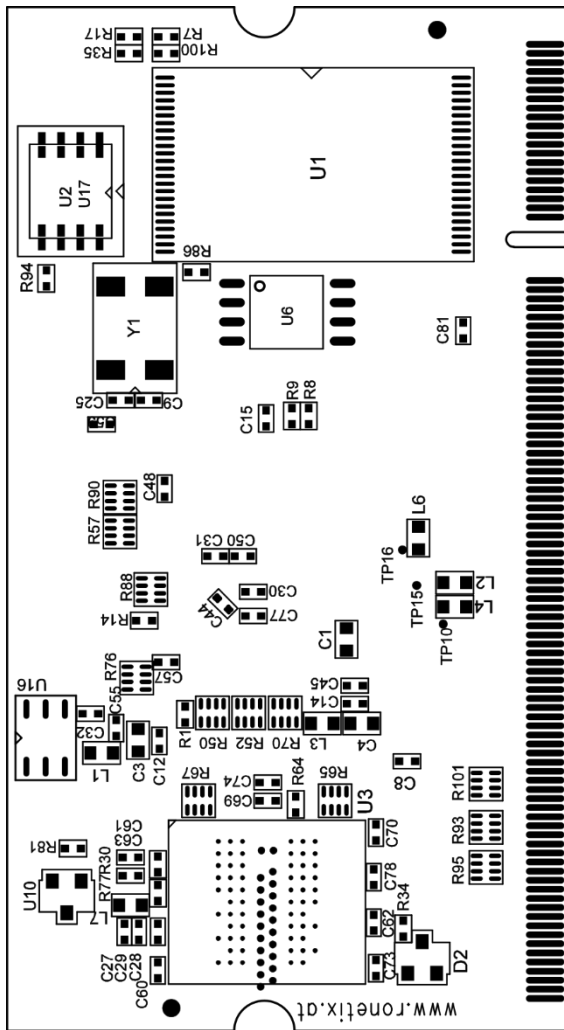
Figure 3: PM9G45 v1.3 bottom
